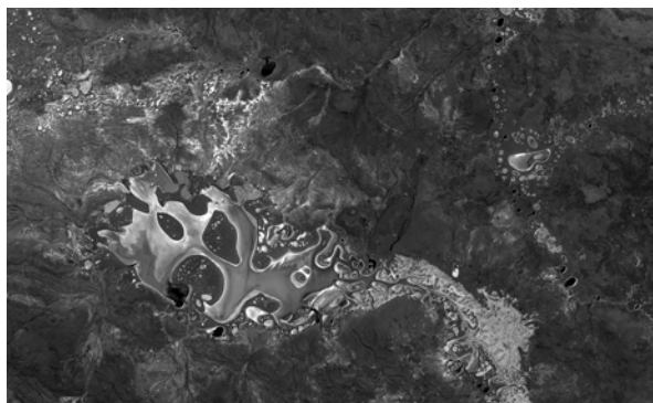
c. Red channel (band 4: 0.636–0.673 \mu\text{m} )
