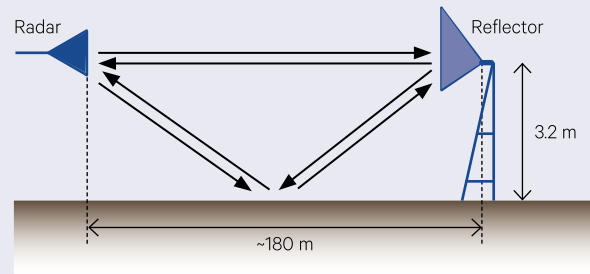
Figure 3.16 Corner reflectors
